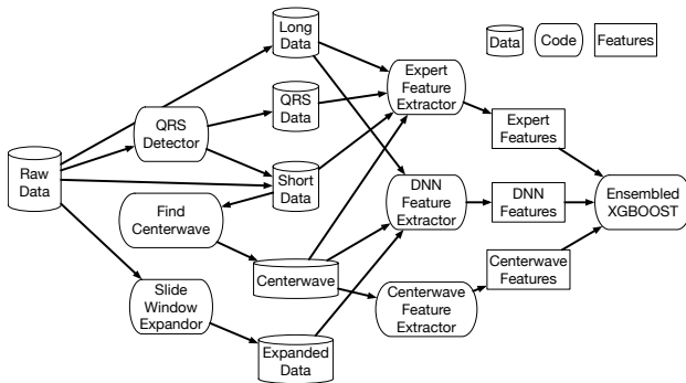
Figure 1. Framework of ENCASE
