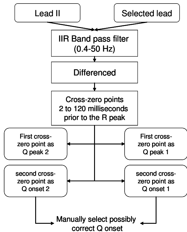
Figure 2. The procedure for finding Q wave and Q onset on lead II and manually selected lead.
