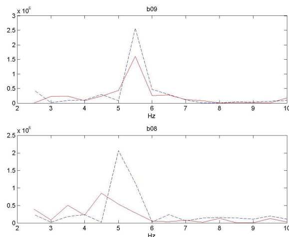
Figure 4: The FFT spectra of the penultimate (dashed) and last (continuous line) two seconds of the couple b08/b09.
