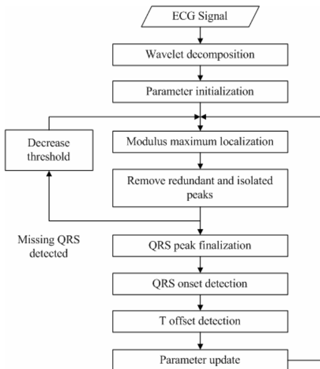
Figure 3. Flow chart for wavelet based QT measurement.
